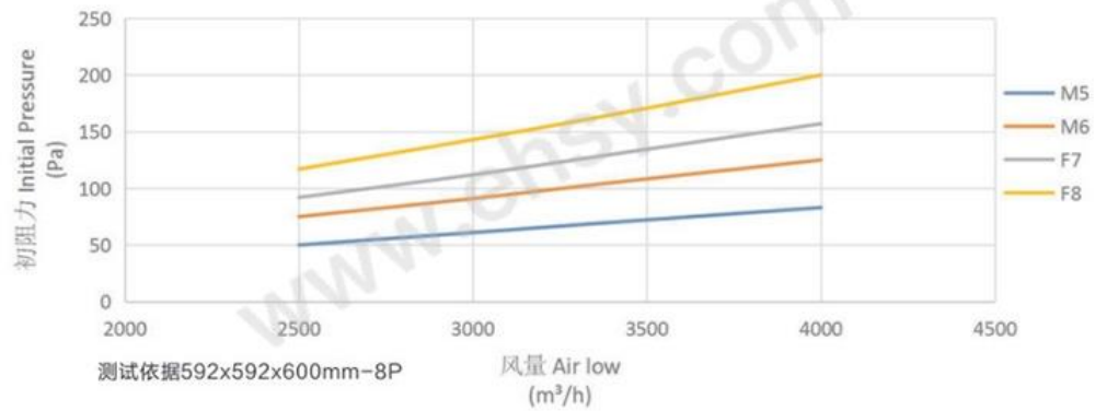
► 初阻力与风量关系曲线图 Relationship between resistance and Air flow
